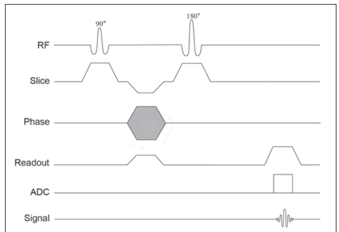
Fig. 2 —Diagram shows steady-state free precession pulse sequence. RF = radiofrequency pulse, ADC = analog-to-digital converter.
